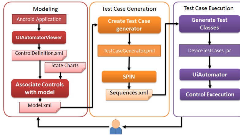
Figure 1: Test generation and execution process
